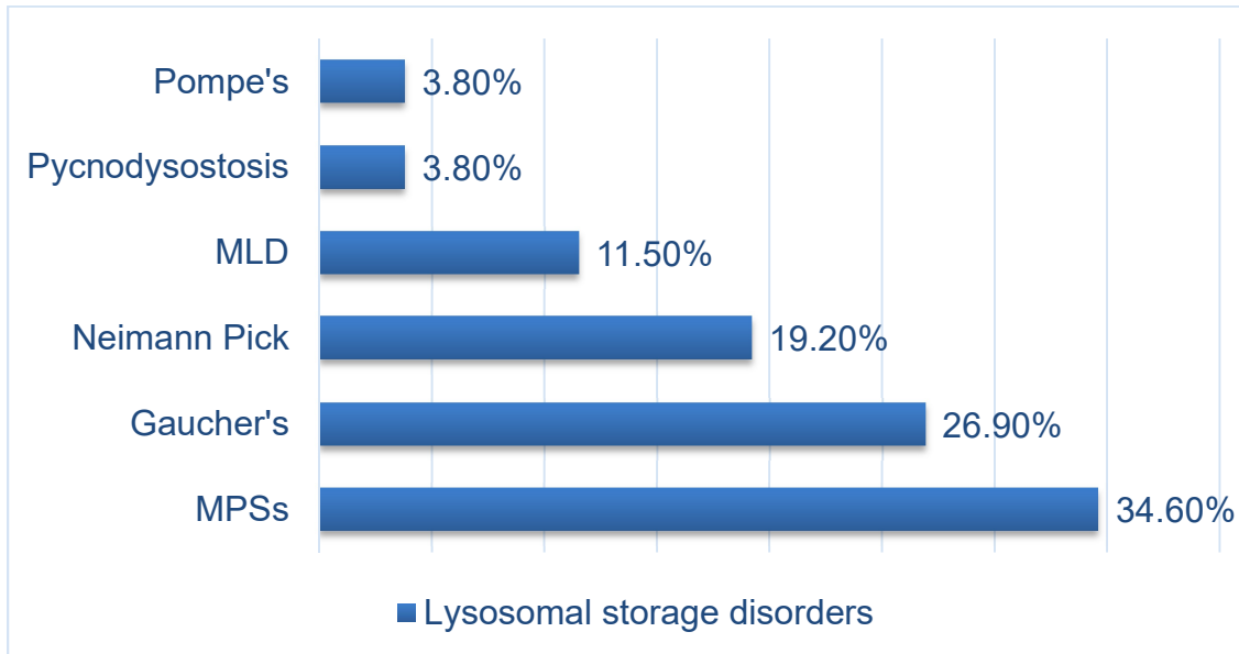
Figure I: Types of Lysosomal storage disorders
