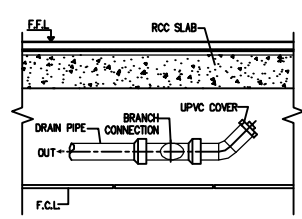
2 DETAIL OF CEILING TYPE CLEAN OUT PLUG (COP) NTS
