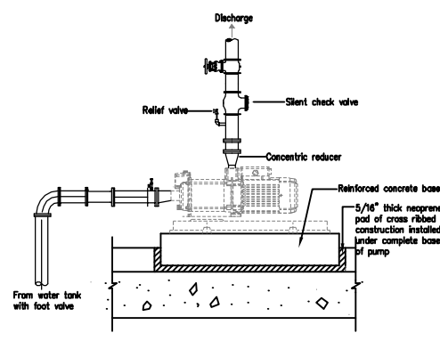
13 TRANSFER PUMP DETAIL NTS
