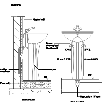
13 LAW - PEDESTAL TYPE NTS
