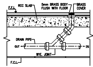
1 DETAIL OF FLOOR CLEAN OUT PLUG (FCO) NTS
