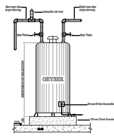
4 DETAIL OF WATER HEATER CONNECTION NTS
