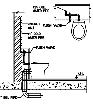
6 DETAIL OF WATER CLOSET CONNECTION NTS
