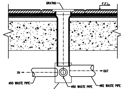
3 DETAIL OF MULTI FLOOR TRAP WITH GRATING NTS
