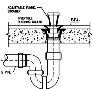
5 BODY W/STRAINER W/ROUND FUNNEL EQUIPMENT FLOOR DRAIN NTS
