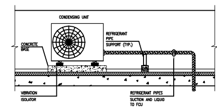
7 INSTALLATION OF SPLIT AC UNIT NTS
