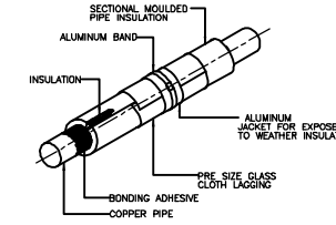
4 PIPE INSULATION DETAIL SCALE N.T.S
